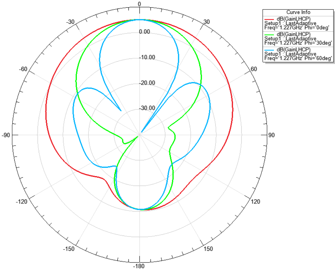
Gain Plot 9
